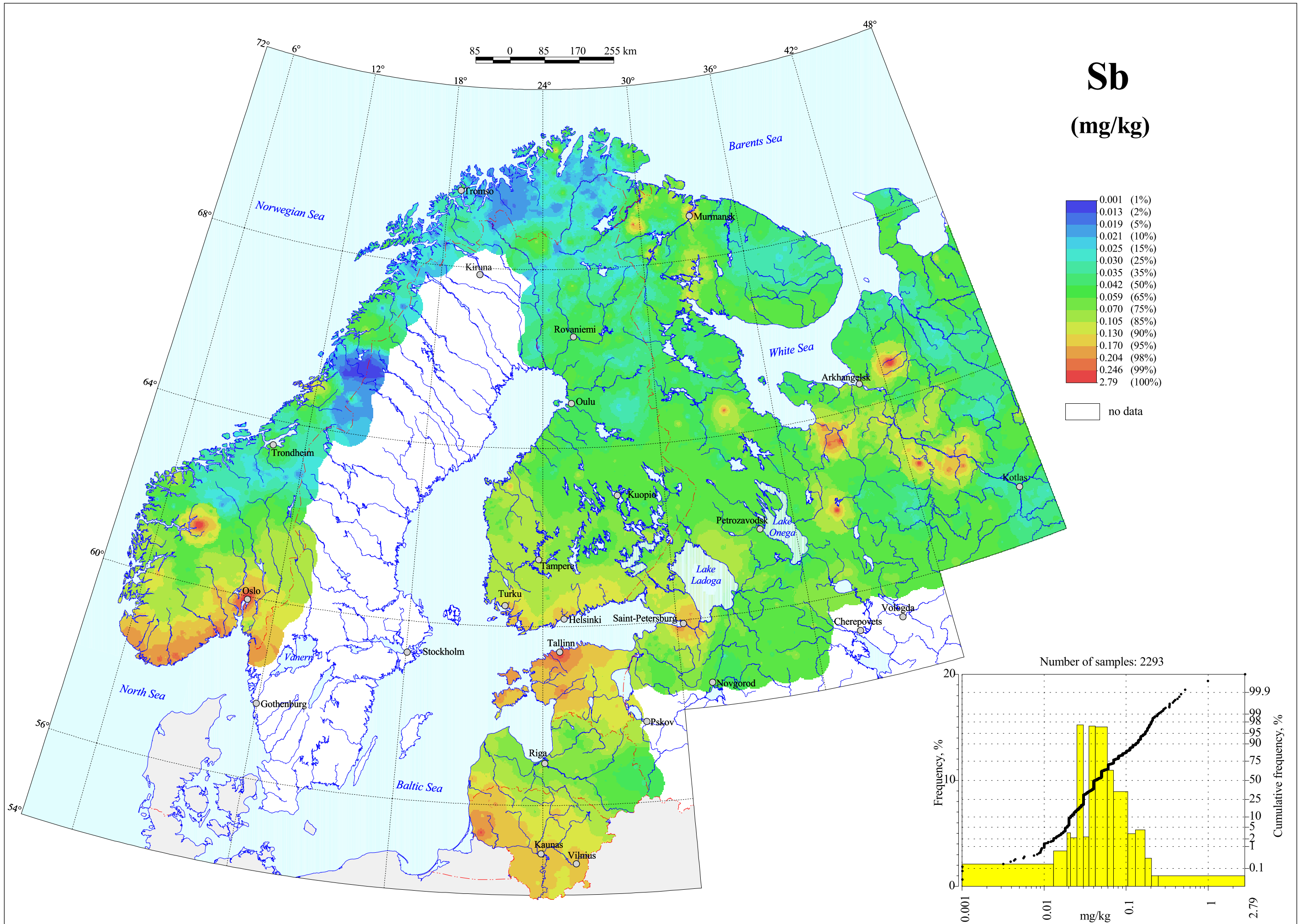
Antimony in Terrestrial Moss, Total Content
